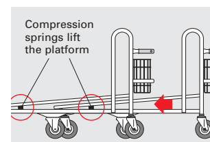
Compression springs under the platform lift the platform for easy and gentle nesting.
