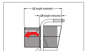
Sliding basket
